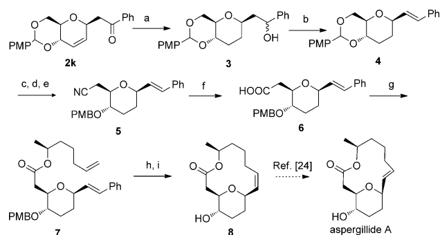
Scheme 5. Formal total synthesis of aspergillide A. Reagents and conditions: a) Raney Ni, H 2 , EtOH/EtOAc 2:1, RT, 95%; b) DTBMP, Tf 2 O, CH 2 Cl 2 , RT, 83%; c) DIBAL-H, CH 2 Cl 2 , -15 °C, 82%; d) TsCl, Et 3 N, DMAP, RT, 91%; e) KCN, DMSO, 50 °C, 79%; f) KOH, EtOH/H 2 O 1:1, 80 °C, 87%; g) ( S )-hept-6-en-2-ol, Yamaguchi esterification, 94%; h) Ru-II, BQ, toluene, 100 °C, 71%; i) DDQ, aq CH 2 Cl 2 , 90%. DDQ = 2,3-dichloro-5,6-dicyano-1,4-benzoquinone, DMAP = 4-dimethylaminopyridine, DTBMP = 2,6-Di- tert -butyl-4-methylpyridine, Ru-II = 2nd generation Grubbs catalyst, Tf = trifluorosulfonyl, Ts = p -toluenesulfonyl.
