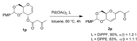
Scheme 4. Decarboxylative coupling of compound 1p .
