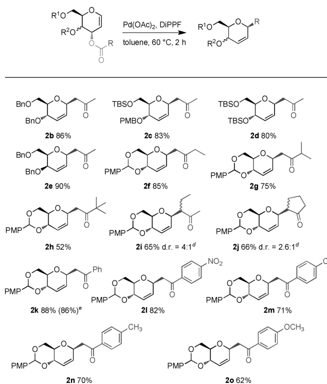
Scheme 2. Decarboxylative glycosylation of glycal-derived β-keto esters. [a–c] [a] Reactions were carried out on a 0.2 mmol scale in the presence of 0.01 mmol Pd(OAc) 2 and 0.02 mmol DiPPF in 2 mL toluene at 60 °C for 2 h. [b] Yield of isolated product. [c] PMP = 4-methoxyphenyl. [d] d.r. was determined by 1 H NMR analysis. [e] Yield for a gram-scale reaction.
