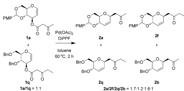
Scheme 3. Crossover decarboxylative coupling of 1a and 1q .
